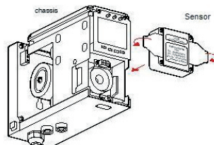
Diagram 3. Fitting/replacing sensor cartridge
