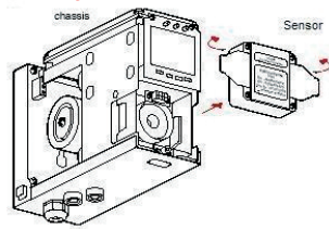
Diagram 2. Removing sensor cartridge
