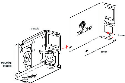
Diagram 1. Removing detector cover
