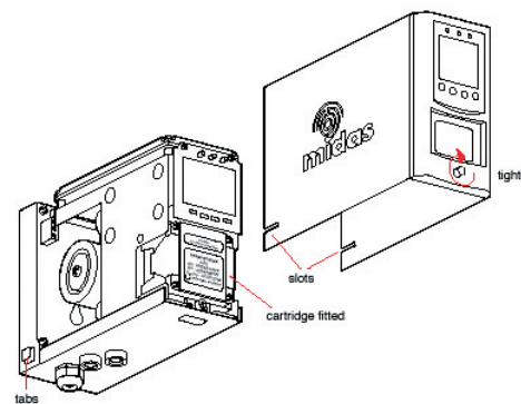
Diagram 4. Refitting detector cover
